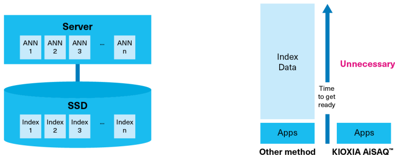
Figure 3: Additional benefits of AiSAQ technology
