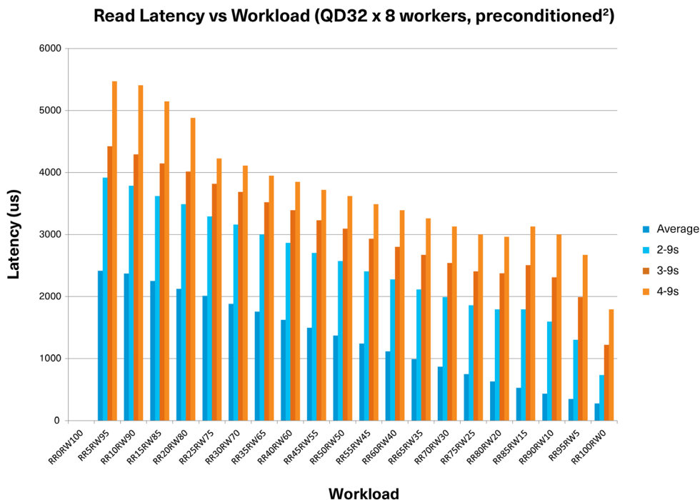
Figure 2: XD6 Series read latency on mixed workloads
