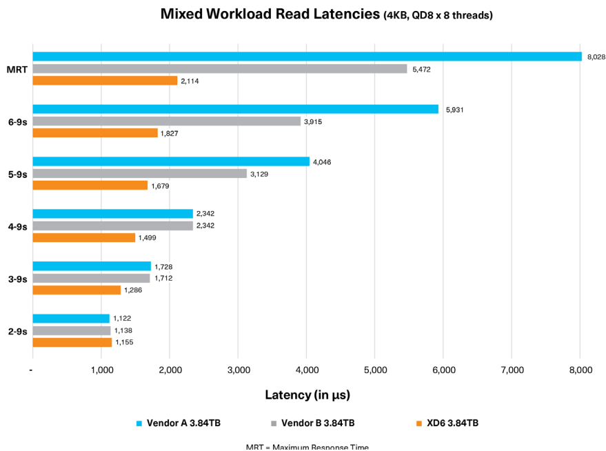
Figure 3: Mixed workload read latency QoS comparing the XD6 Series to two U.2 SSDs from leading vendors
