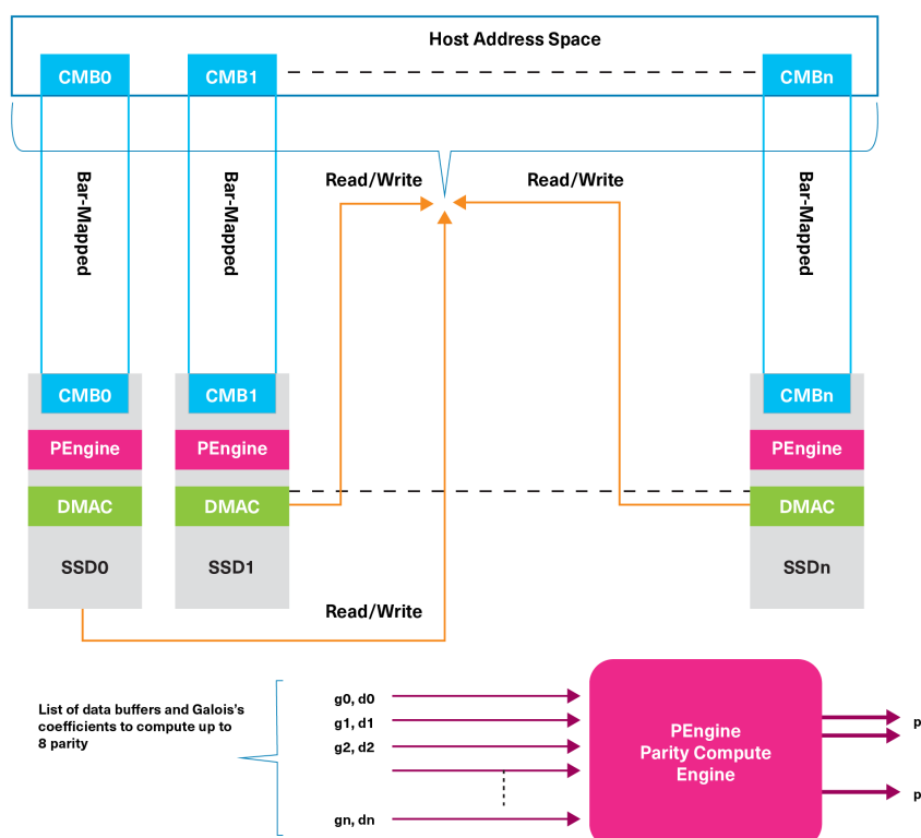
Figure 3 depicts the SSD RAID Offload construct
